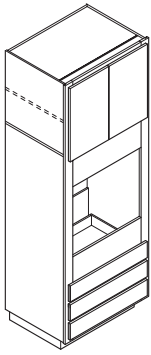
SINGLE OVEN 3 DRAWERS 93" HIGH
