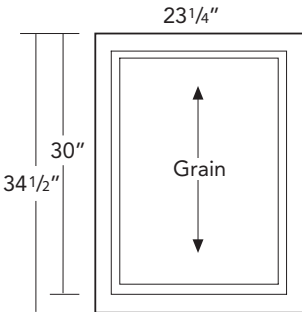
BASE END PANEL
