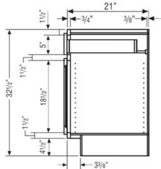
32.5" VANITY BASE CABINET
