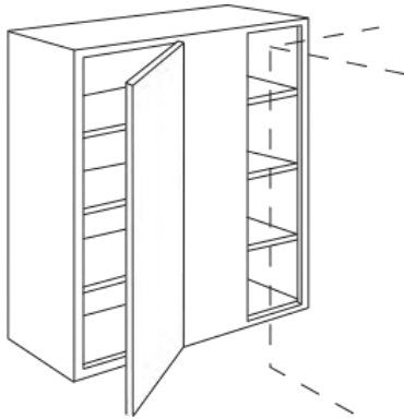
BLIND CORNER SINGLE DOOR 39" HEIGHT
