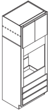
SINGLE/DOUBLE OVEN 3 DRAWERS 90" HIGH
