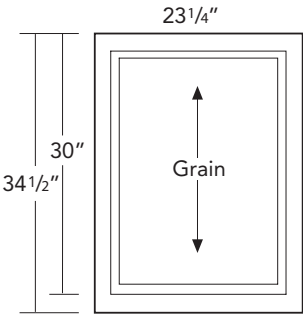
BASE END DECORATIVE DOOR PANEL KIT
