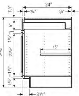
BASE CABINET
