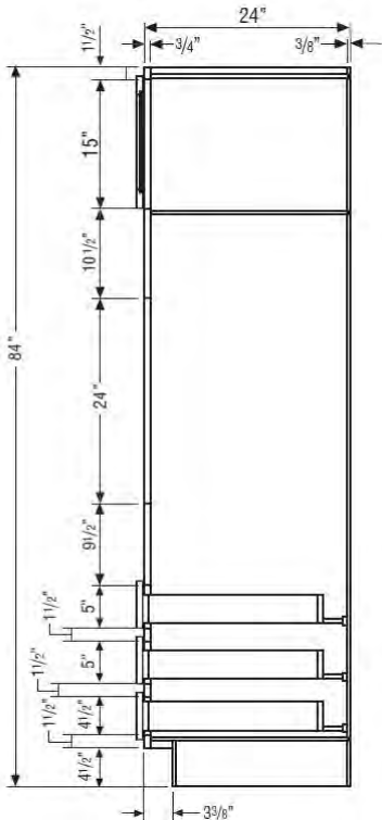
OVEN CABINET
