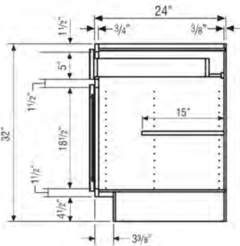
32.5" BASE CABINET
