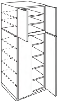
DOUBLE DOOR TALL PANTRY 96" HIGH
