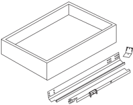
ROLL TRAY KITS
