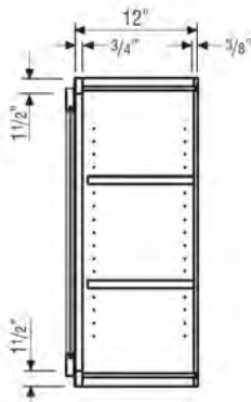
WALL CABINET
