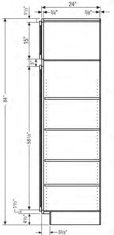
TALL CABINET
